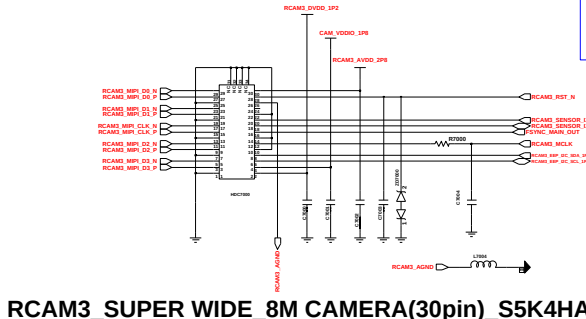
RCAM3_SUPER WIDE_8M CAMERA(30pin)_S5K4HA
