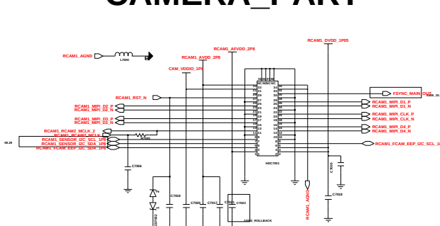
RCAM1_24M CAMERA(34PIN)_IMX576
