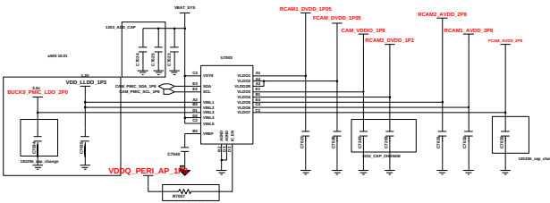
CAM PMIC
