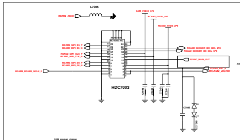
RCAM2_5M CAMERA(24PIN)_GC5035
